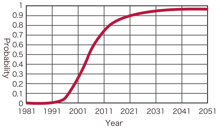
Miyagi Earthquake Reoccurrence Probability Interval (Estimate) (Headquarters for Earthquake Research Promotion)
